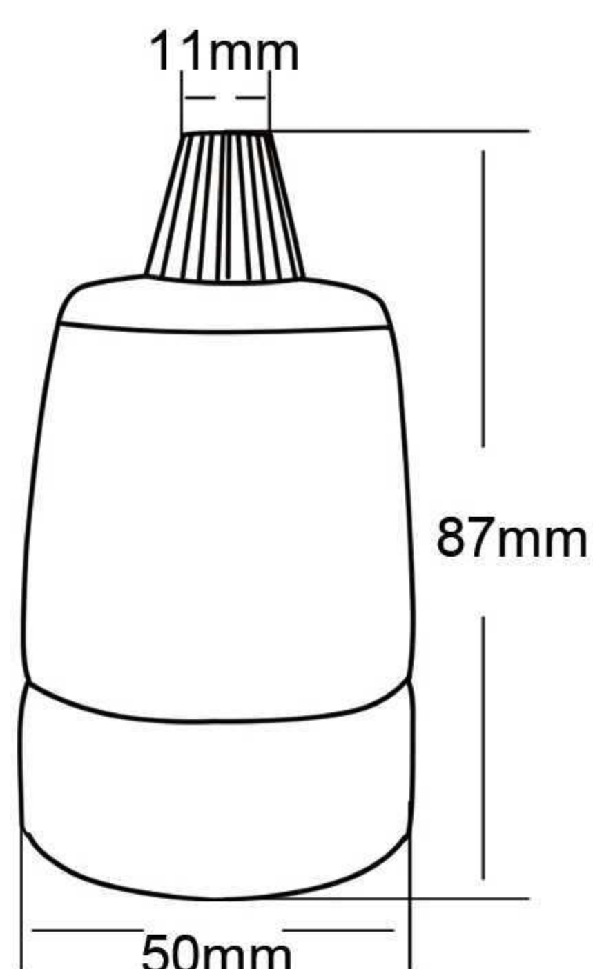
Silicon lampholder
